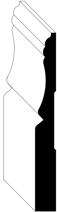
#5220 Colonial Base 7/16" x 4"
