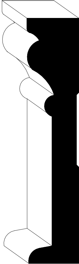
#5500 Boston Header 4 7/16" x 1"
