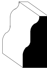
#5311 Bed Mould 1 1/8" x 9/16"
