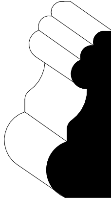
#5270 Chair Rail 1 11/16" x 11/16"
