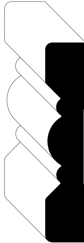
#5110 MacDonald Casing 3 3/8" x 11/16"
